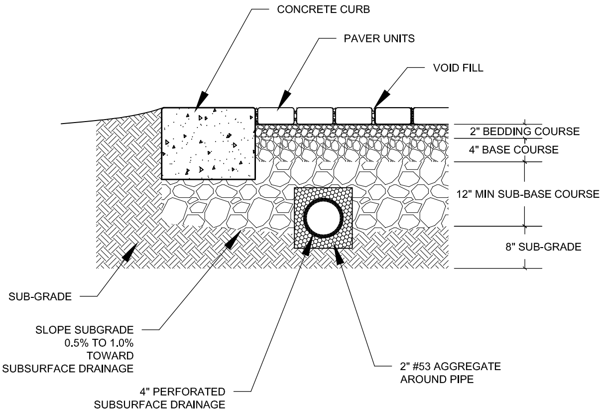
1 D1 PERMEABLE PAVEMENT SYSTEM TYPICAL SECTION NTS
